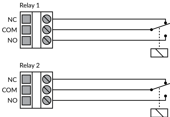
Figure 2b - Wiring diagram relay(s)
