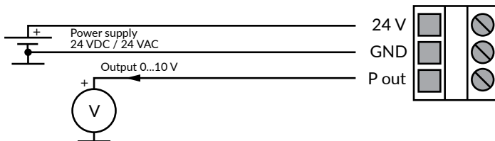
Figure 2a - Wiring diagram 0–10 V output
