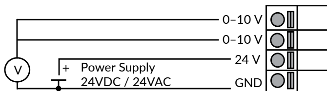
Figure 2 - Wiring diagram
