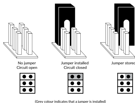
Figure 3 - Jumper installation
