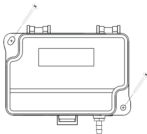
Figure 1a - Surface mounting
