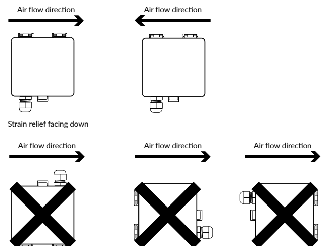
Figure 1c - Mounting orientation
